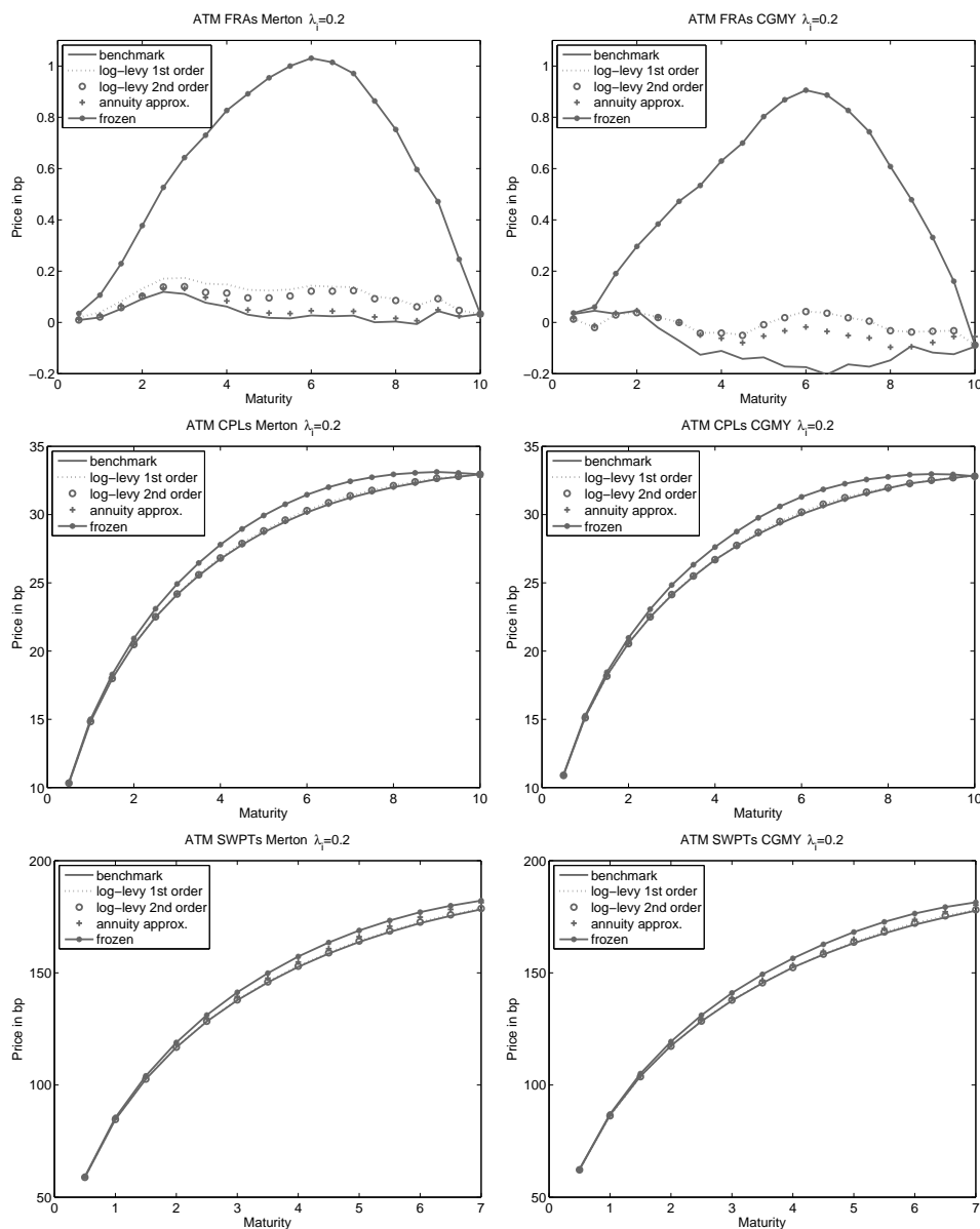
FIGURE 5.3. Prices for the Merton and CGMY models.
